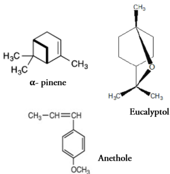
Fig. 1. Molecular structure of the major compounds found in the Pistacia atlantica , Myrtus communis , Foeniculum vulgare and Eucalyptus globulus essential oils.
