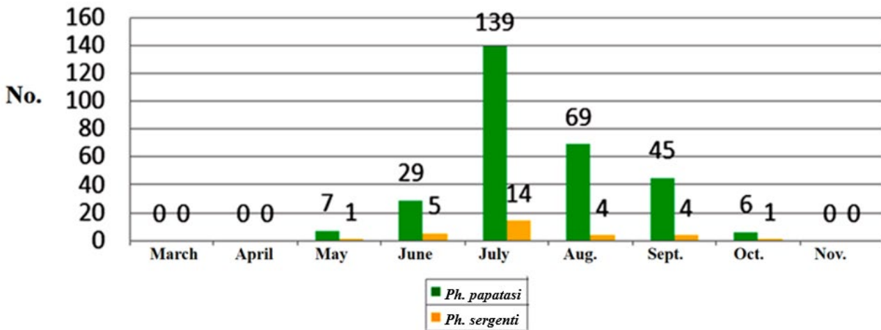
Fig. 2: Abundance and activity of sandflies caught in different months of the year in the Kavirat district of Aran and Bidgol County.
